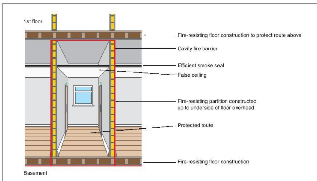
Figure 1: Fire-resisting construction
