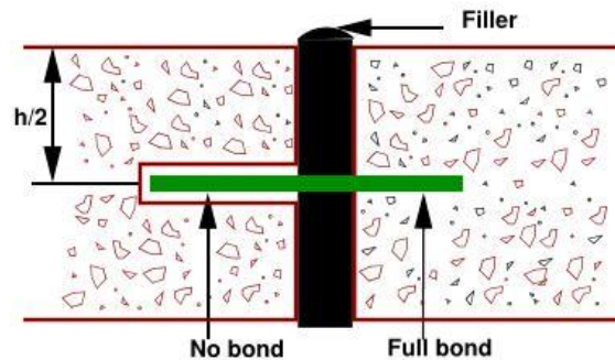
Fig. 35.1 Expansion joint
