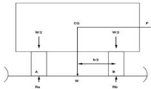
Fig. 7.1. Effect of horizontal curve
