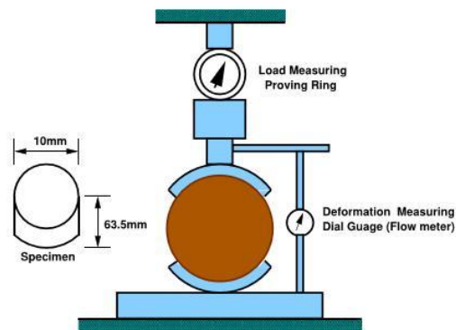
Fig. 30.1 Marshall Mould
