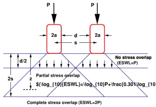
Fig. 31.1 ESWL-Equal stress concept
