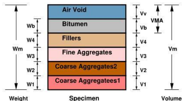
Fig. 30.2 Marshall Mould
