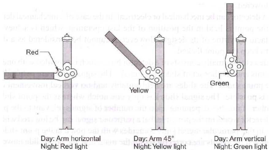
Fig. Upper Quadrant signalling
