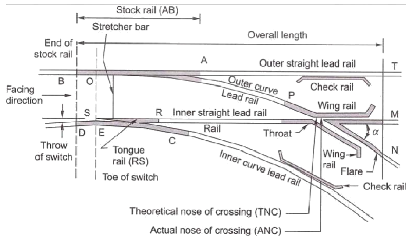
Fig. (a) Constituents of a turnout
