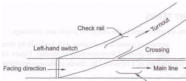
Fig. (b) Left-hand turnout
